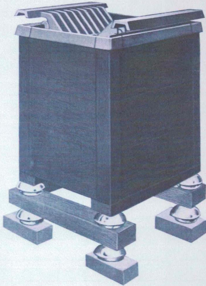
Type "G" 19 Plates in Lead-Lined Wood Tank
