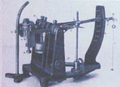
Fig. 2. Signaling Hydrometer
