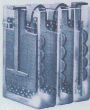
"BT" Couples in Glass Jars
