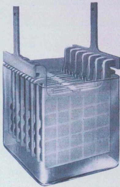
Type "E" 13 Plates in Glass Jar
