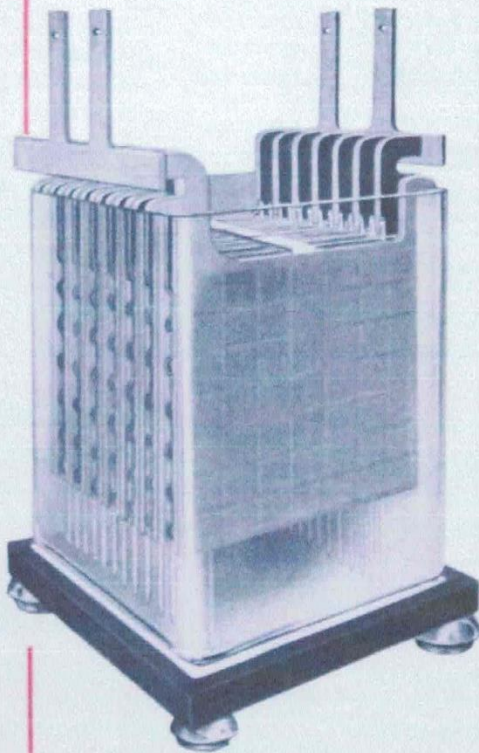
Type "F" 15 Plates in Glass Jar
