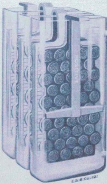
"PT" Couples in Glass Jars
