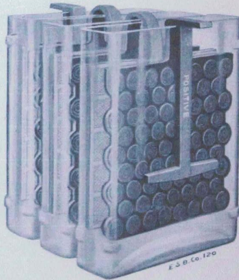
"ET" Couples in Glass Jars
